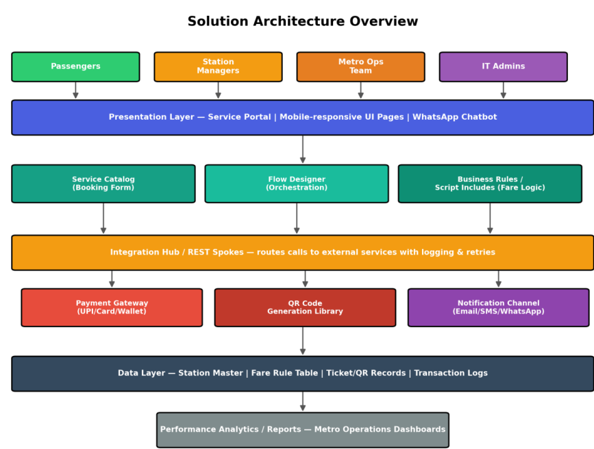
Figure — End-to-end solution architecture on the Now Platform
